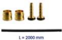
2023016 Hydraulic hose replacement kit 2000mm for Tektro 5.5
