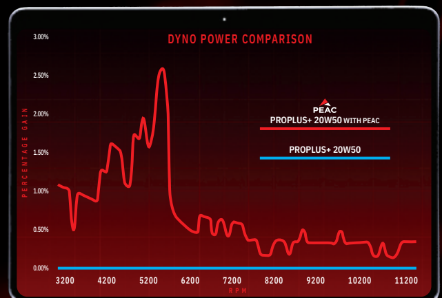
PEAC DYN0 TESTING / PRO PLUS+
