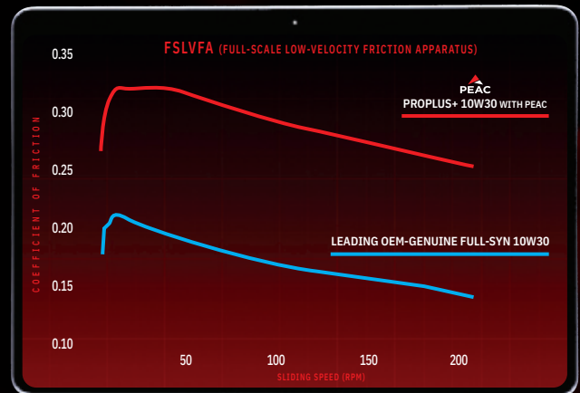
PEAC CLUTCH PERFORMANCE @ 170°C
